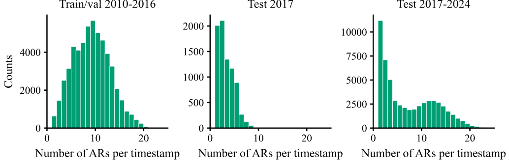
Figure 5: Number of ARs per timestamp across different datasets
