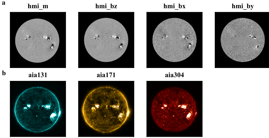
Figure 4: Solar full disk images of four HMI and three AIA channels at 2017/09/07 01:00. hmi_m refers to the line of sight magnetogram.
