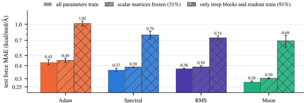
Figure 6: Test force MAE (kcal/mol/Å, \downarrow ) for GotenNet on rMD17 aspirin with all parameters trained, scalar matrices frozen, or only the irrep blocks and readout trained. The number in parentheses is the percentage of parameters frozen at their initial values. Mean and std over three seeds.
