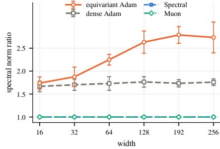
Figure 2: Ratio between the largest and smallest spectral norms of the matrix updates at Adam’s first update. The mismatch increases with width in the equivariant model but remains nearly constant in the matched dense MLP. Spectral and Muon have a ratio of one by construction. Mean and standard deviations over eight seeds.
