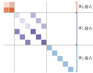
(b) The corresponding expanded map.
