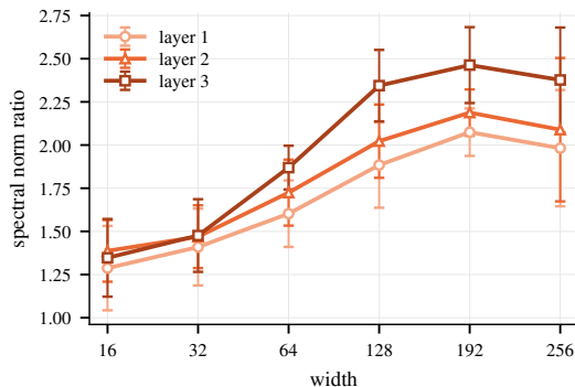
Figure 3: Ratio between the spectral norms of the updates of the scalar and vector irreducible blocks, W_0 and W_1 , in each hidden layer of the equivariant model on the synthetic task, at Adam’s first update. Setting as in Figure 2; mean and standard deviation over eight seeds.
