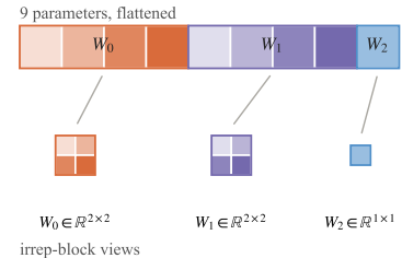
(a) Flat storage and irrep-block views.
